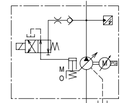
Dual Displacement Type ASR * - * - * W * -
